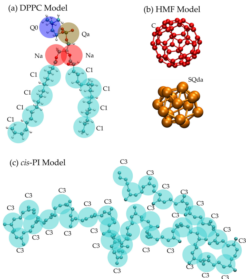
Figure 1. Mapping the atomistic model onto the CG model for cis -PI, DPPC, and HMF molecules: (a) DPPC model with CG bead type names Q0 (charged), Qa (charged), Na (nonpolar), and C1 (apolar) connected beads; (b) pristine fullerene and HMF with CG bead type names SQda (charged) interconnected beads; (c) rubber chain with atom type name C3 (apolar) connected to form a chain. Note that: the bead types Q0, Qa, Na, and C1 are adopted from the standard MARTINI force field [42].
